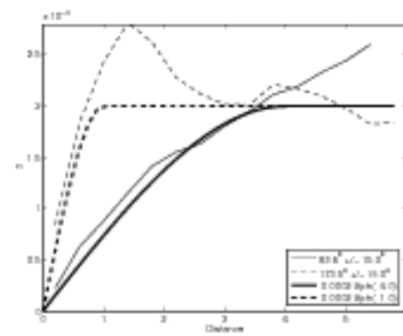
(f) dssim reference semivariogram
