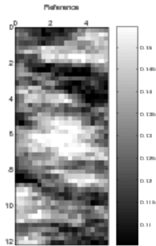
(a) sgsim reference model
