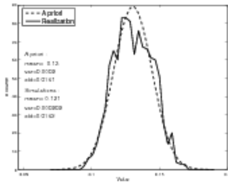
(c) sgsim reference histogram
